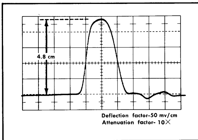
Fig. 2-18. Voltage measurement from display. Example: 4.8 \text{ cm} \times 50 \text{ mv/cm} \times 10\text{X} = 2.4 \text{ v} .
