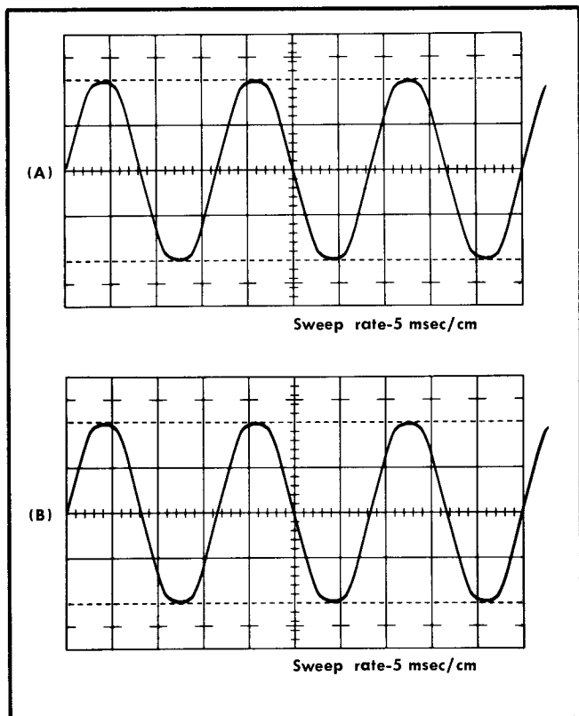
Fig. 2-17. Crt displays showing comparison between real-time sampling and non-sampling presentations of a 60 cps waveform. (A) Waveform obtained with Type 151; (B) Waveform obtained with non-sampling plug-in unit.
