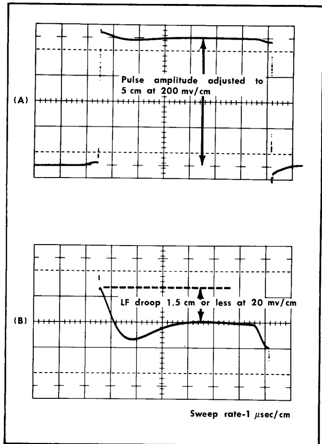
Fig. 5-46. Typical indicator oscilloscope displays for checking low-frequency droop.
