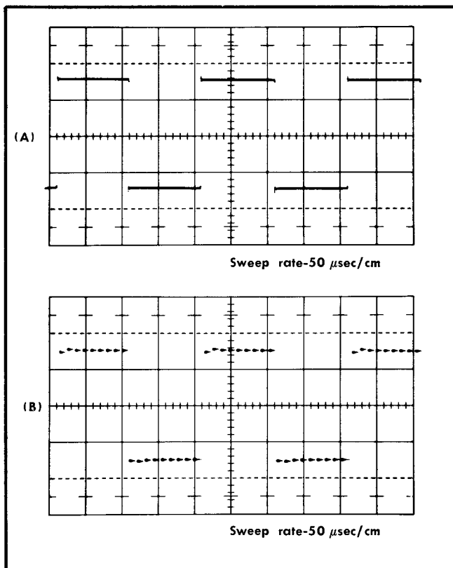
Fig. 2-16. Crt display of a 5-kc square wave showing comparison between equivalent-time sampling (A) and real-time sampling (B), just past the sweep-rate limit of real-time sampling (see text).
