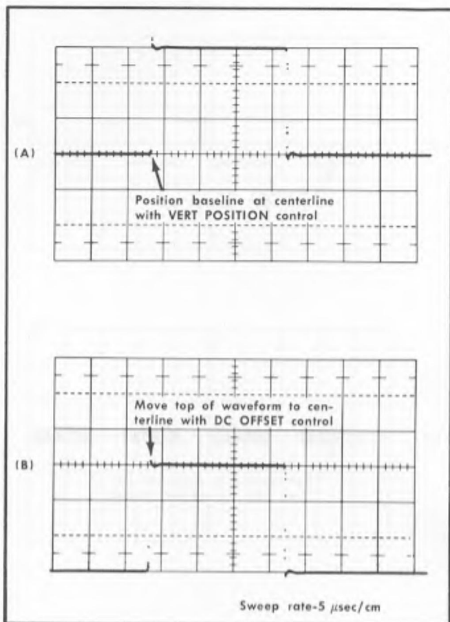
Fig. 5-41. Typical indicator oscilloscope displays obtained during check of offset output.
