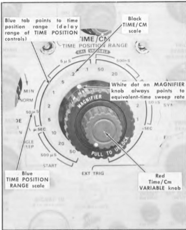
Fig. 2-11. Use of the time magnifier for expanding the display. As shown, the unit is set for \times 5 magnification with a display sweep rate of 0.2 \mu\text{sec}/\text{cm} and a crt "time window" positioning range of 50 \mu\text{sec} .
