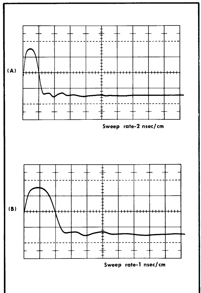
Fig. 2-3. Typical oscilloscope display illustrating time magnification of the display. Expansion takes place about the left edge of the screen.
