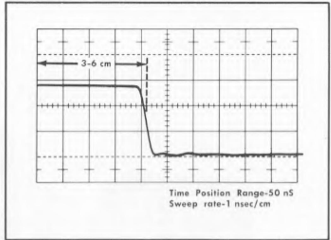
Fig. 5-23. Typical indicator oscilloscope display for checking adjustment of R370 (DELAY ZERO).
