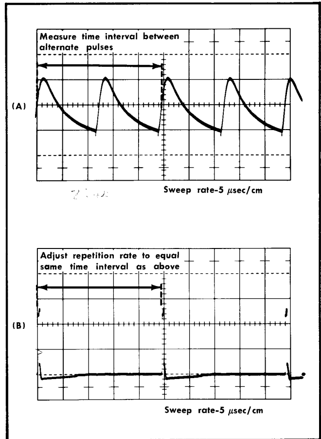
Fig. 5-30. Typical test oscilloscope displays for adjusting pretrigger pulse generator repetition rate to produce 2 trace sampling display. (A) Waveform at Type 1S1 HORIZ OUTPUT (B) pretrigger pulse of pretrigger pulse generator.
