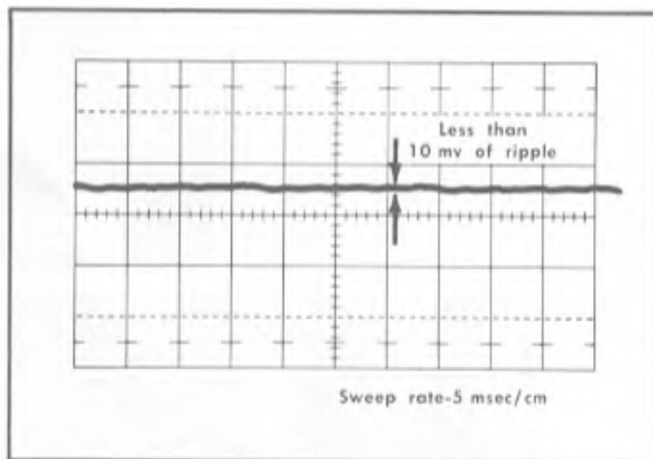
Fig. 5-6. Typical test oscilloscope display of power supply ripple at -19-volt or +19-volt test point (with trigger circuit not free running).
